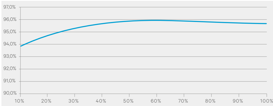
Liebert NXC efficiency curve
