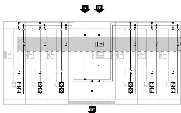
MODULYS XL hybrid bypass architecture:
